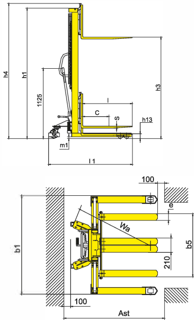
SDJAS series with Straddle legs and adjustable forks
