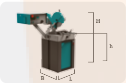
VELOX 350 SHE B 1100 mm L 920 mm H 1700 mm h 265 mm Kg 266
