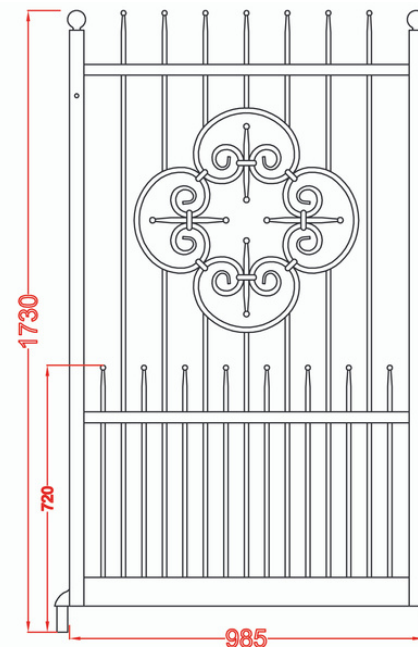
Cancela peatonal
