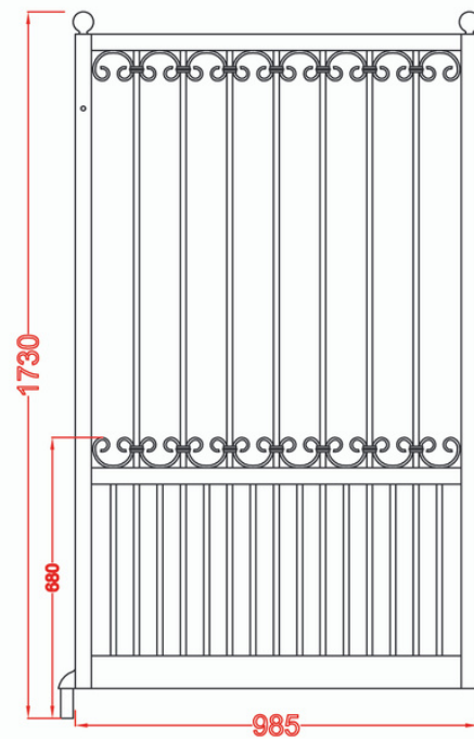
Cancela peatonal
