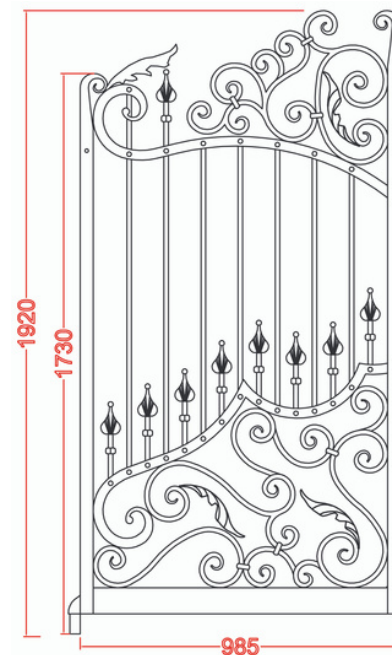
Cancela peatonal
