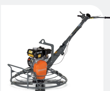
GASOLINA HUSQVARNA BG 375 3.6–6.3 kW, 900 mm, 88–102 kg.
