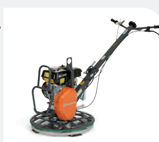
GASOLINA HUSQVARNA BG 245 2.5 kW, 600 mm, 58 kg.
