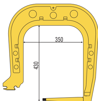
CA6 ARM + ELECTRODE L=430 mm - 803187
