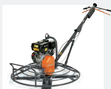
PETROL-POWERED HUSQVARNA BG 475 6.3 kW, 1140 mm, 105 kg.
