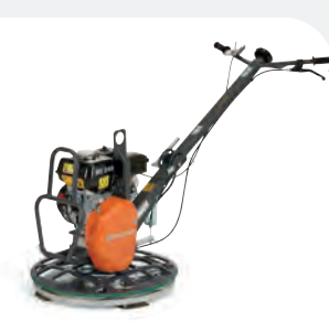
PETROL-POWERED HUSQVARNA BG 245 2.5 kW, 600 mm, 58 kg.
