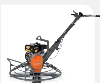
PETROL-POWERED HUSQVARNA BG 375 4.3–6.3 kW, 900 mm, 93–102 kg.
