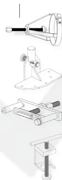
Secondary shaft pulley puller
