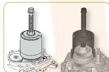
Bearings puller set for automatic transmission gear box - VAG group
