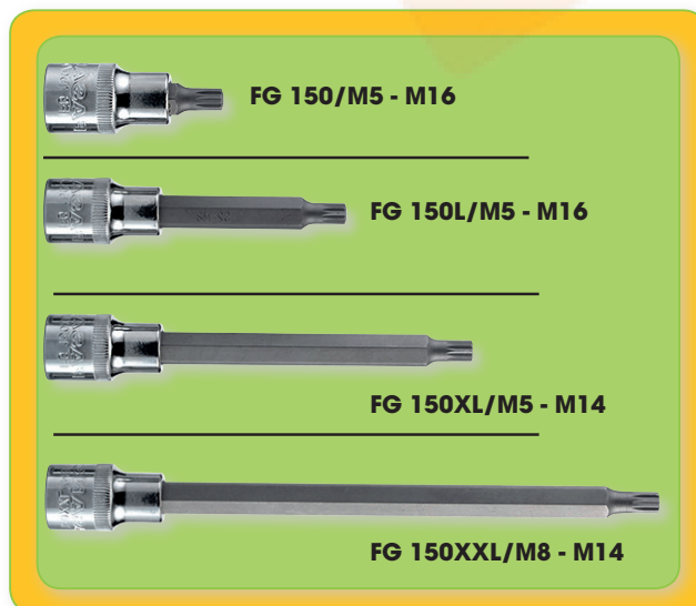
Set 1/2"dr. 26pcs socket bits - XZN
